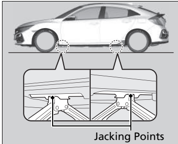
Jacking Points
