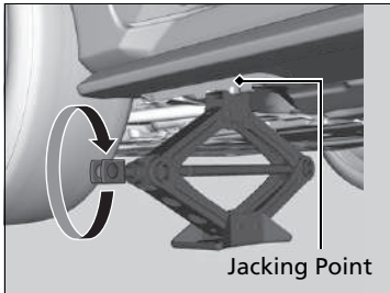
Jacking Points
