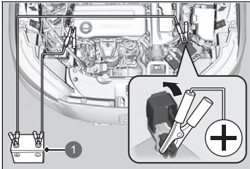
1 Booster Battery
